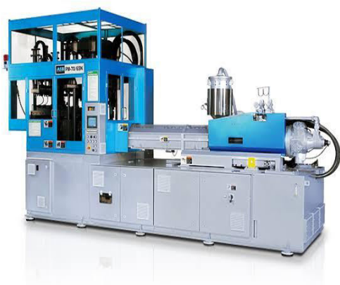
ASB PET Preform Machine
